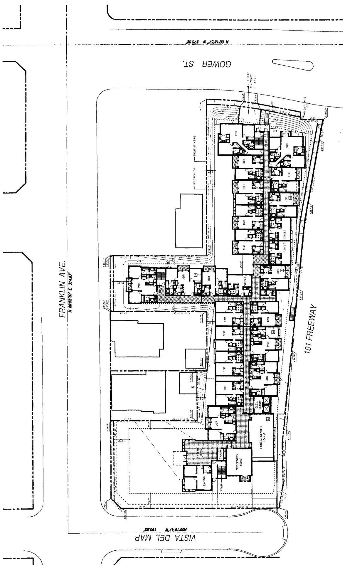
Figure III-2 Proposed Site Plan
