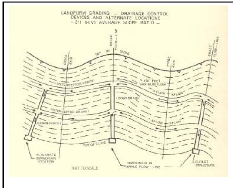
Figure 2 - Landform Grading
