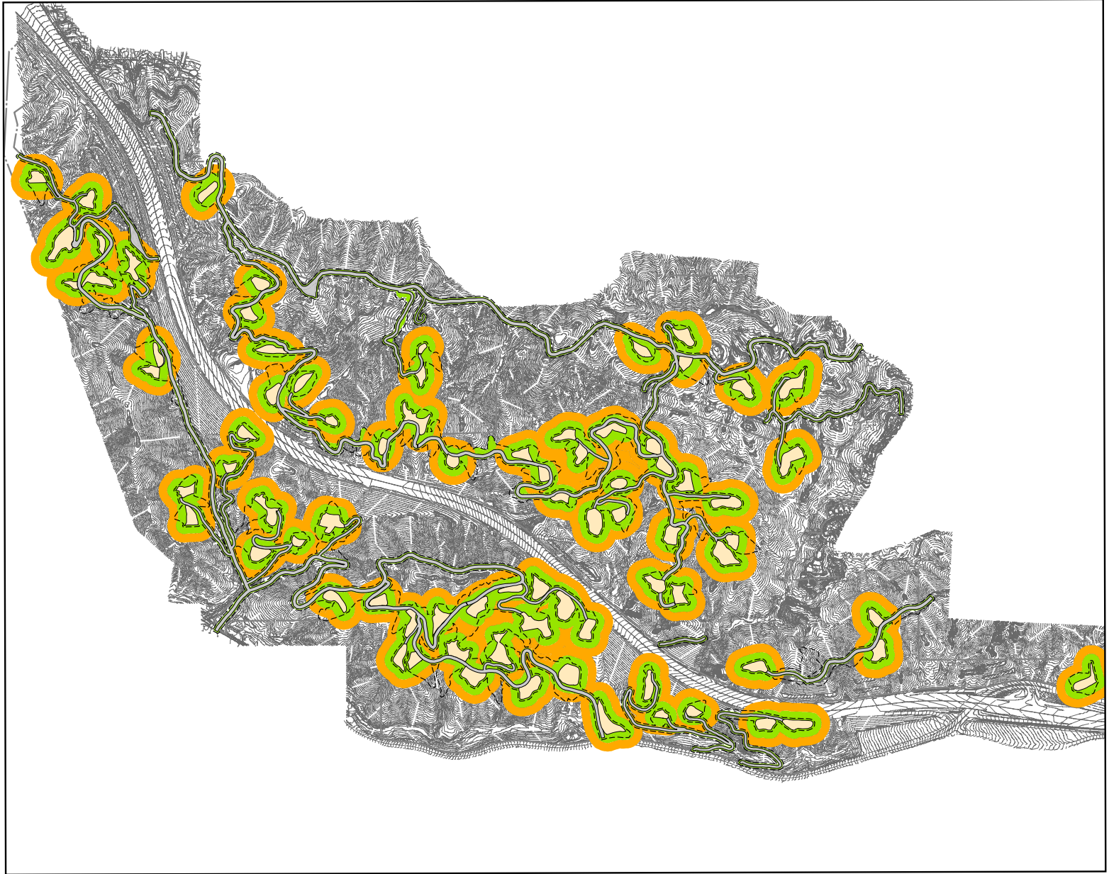
Figure VI-4 Grading Limits, Brush Clearance, and Fuel Modification Zones for 87 Lot Alternative Plan
