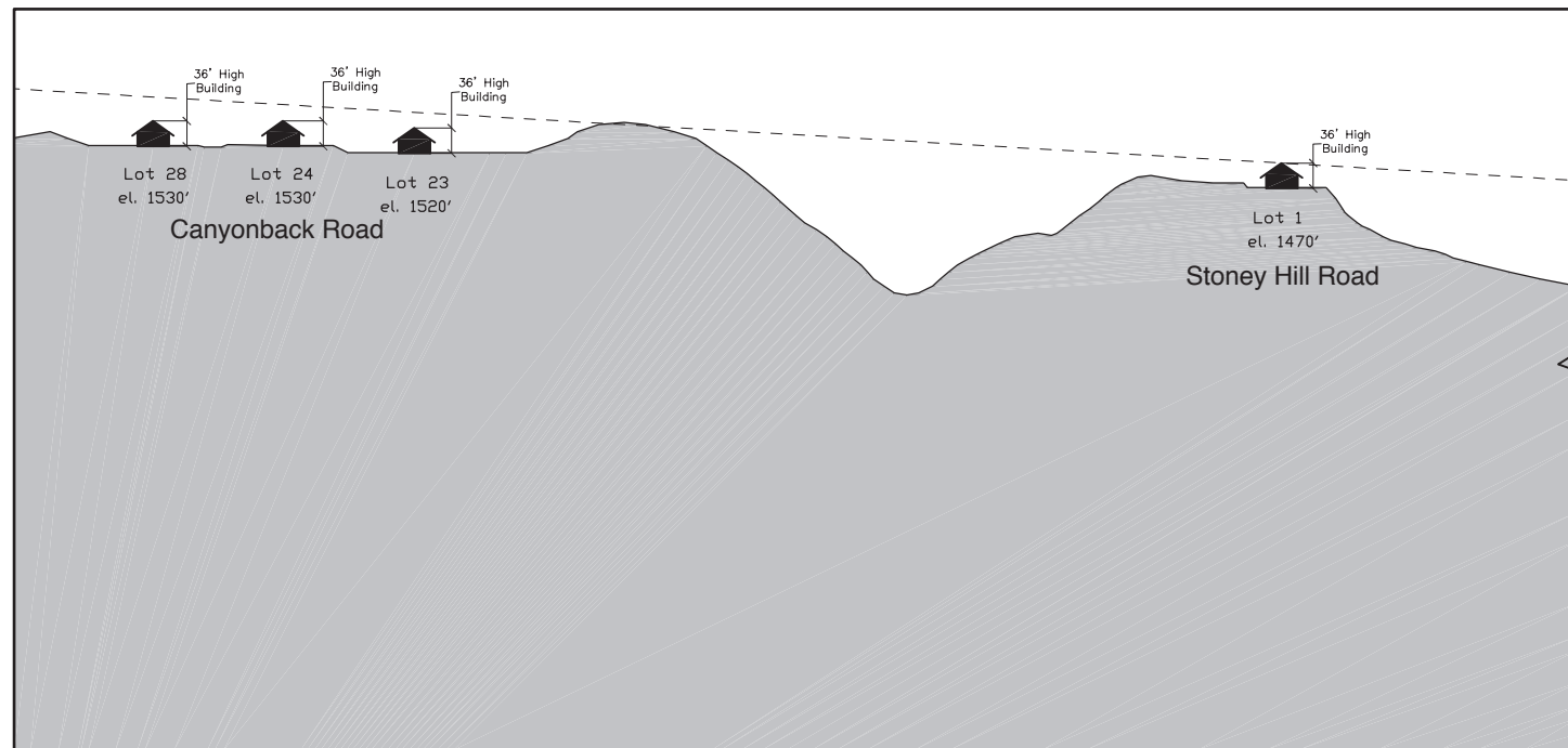
Section AA
