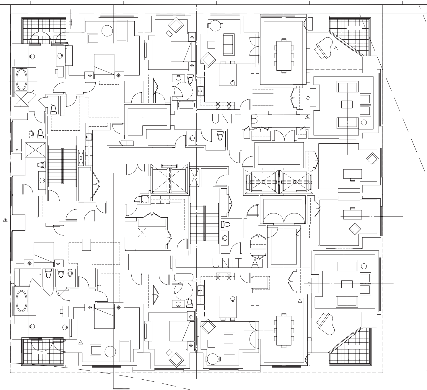
Figure III-3 Proposed Site Plan: 3-5th Floors
