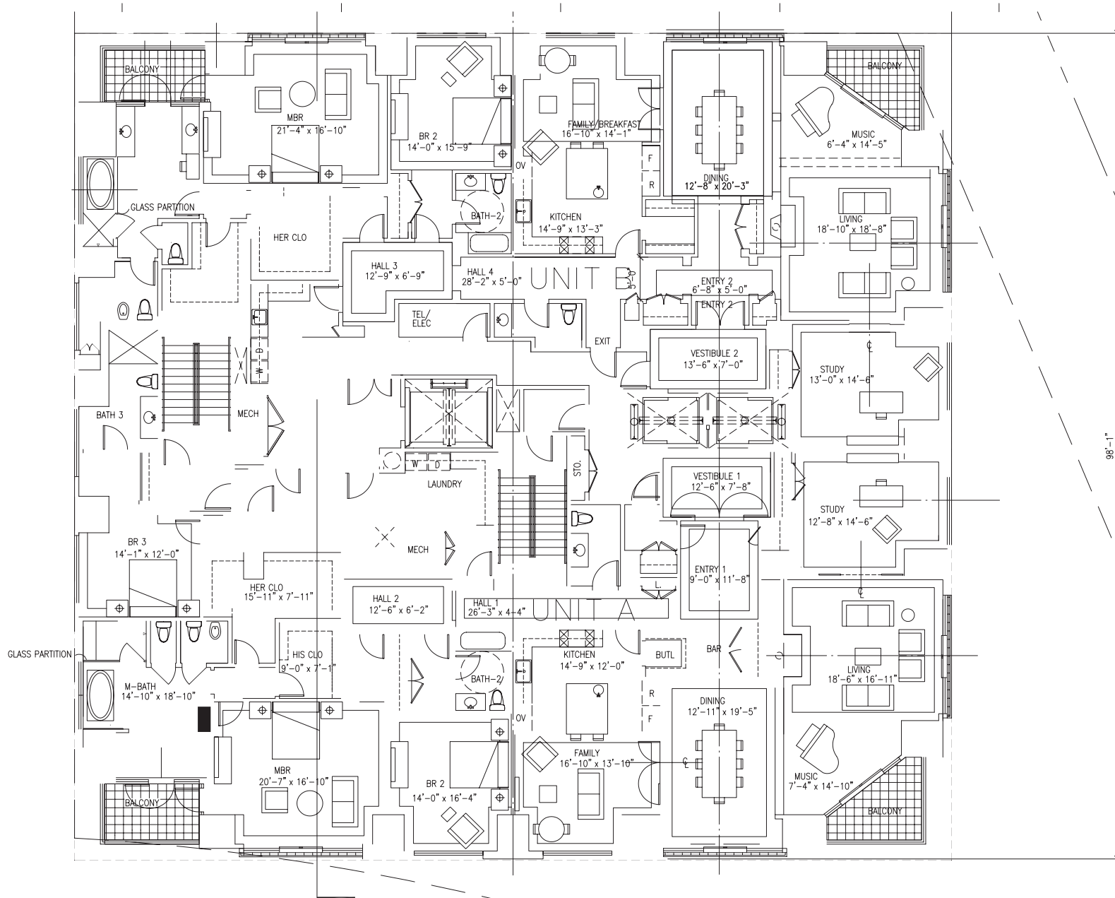
Figure III-4 Proposed Site Plan: 6-10th Floors
