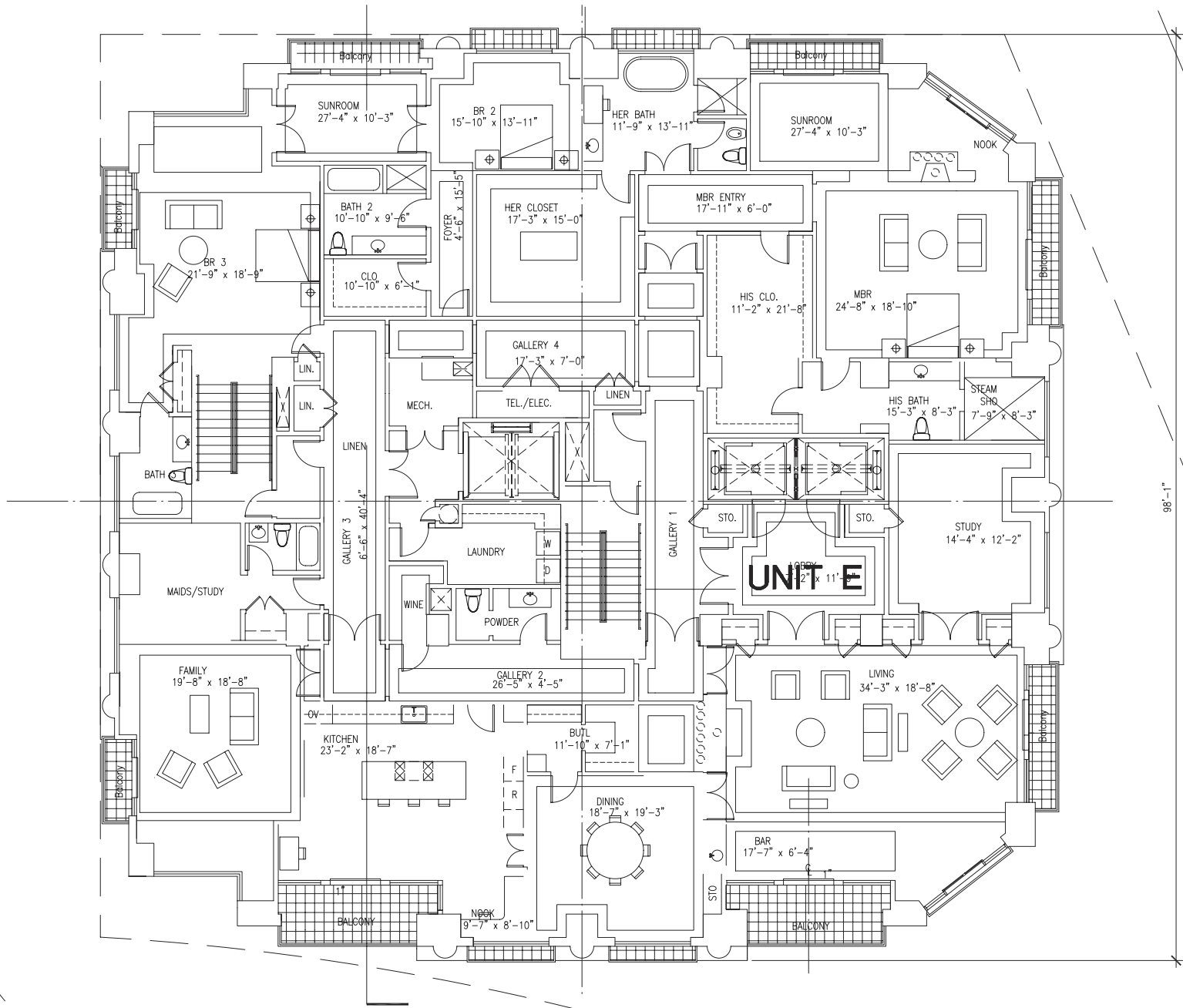
Figure III-8 Proposed Site Plan: 21st Floor
