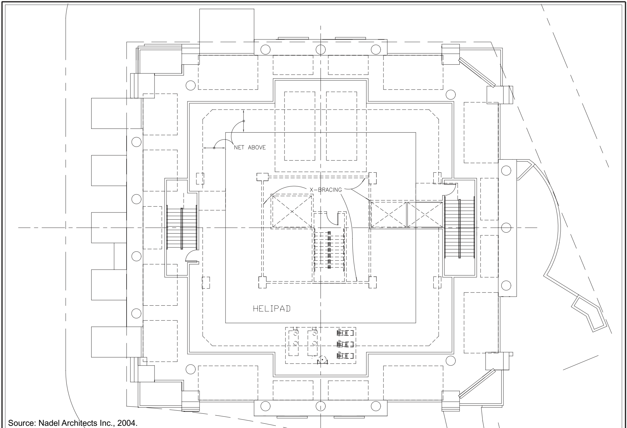
Figure III-9 Proposed Site Plan: Roof
