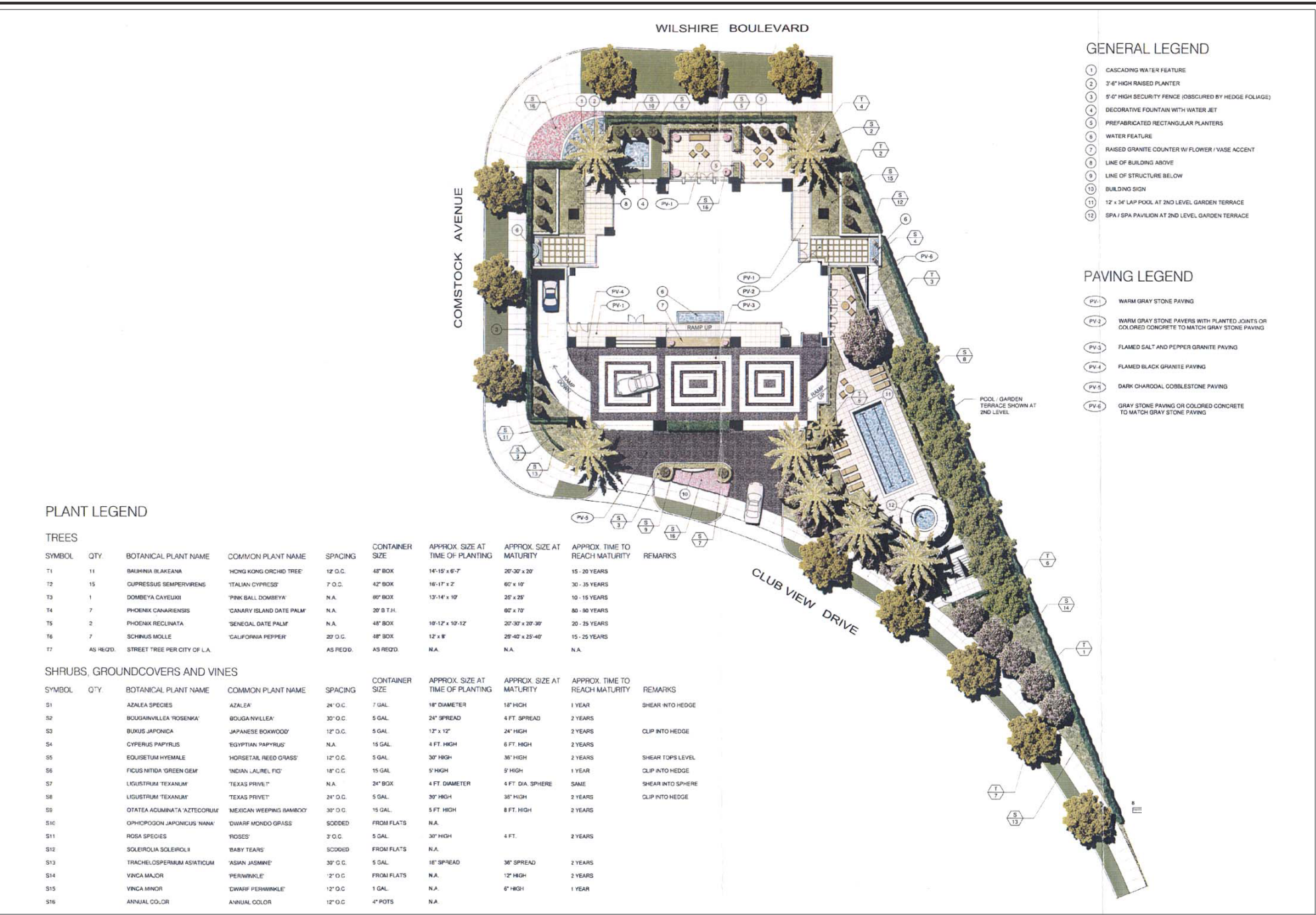
Figure III-18 Proposed Project Landscape Plan
