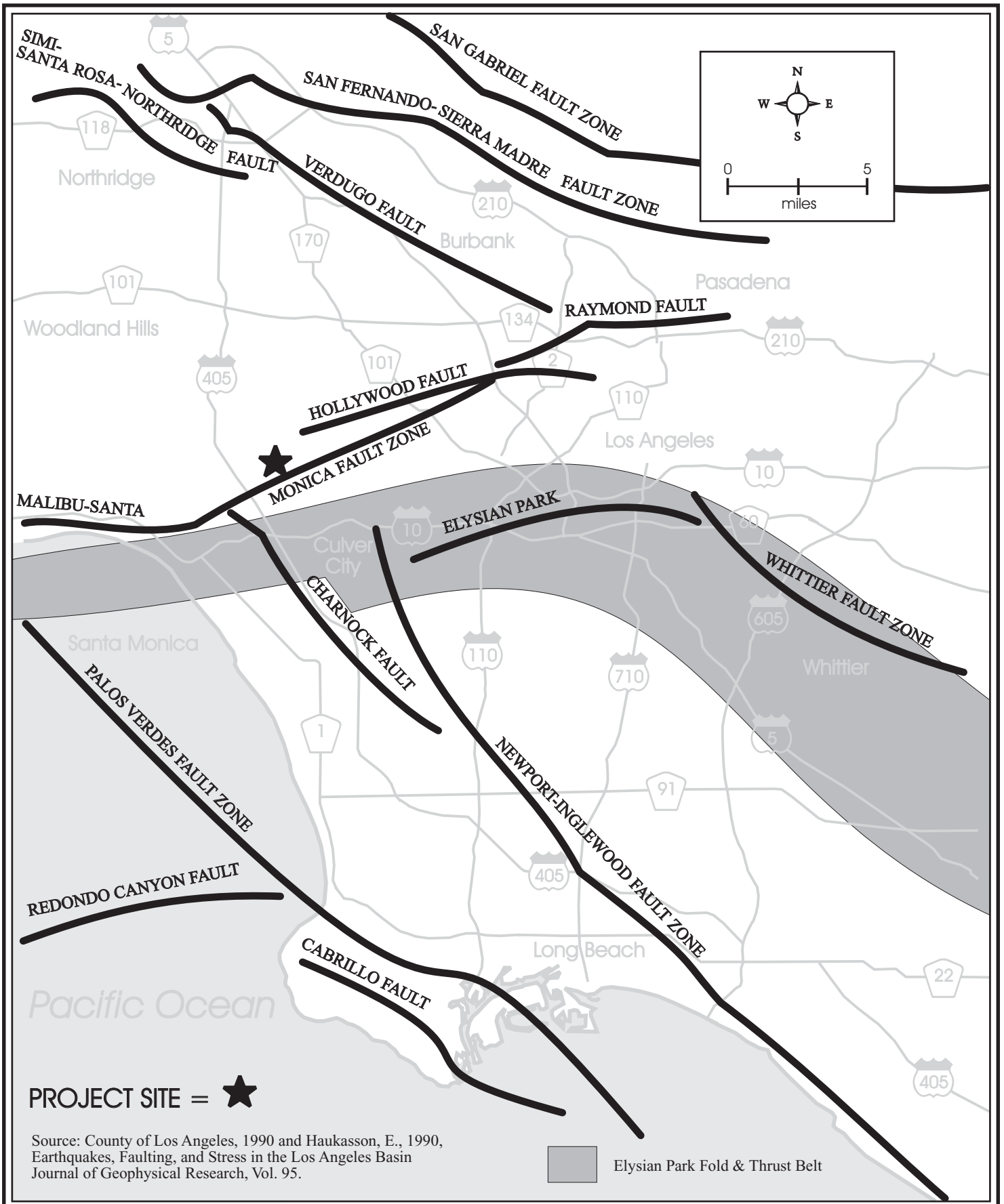
Figure IV.D-2 Regional Faults and Seismicity
