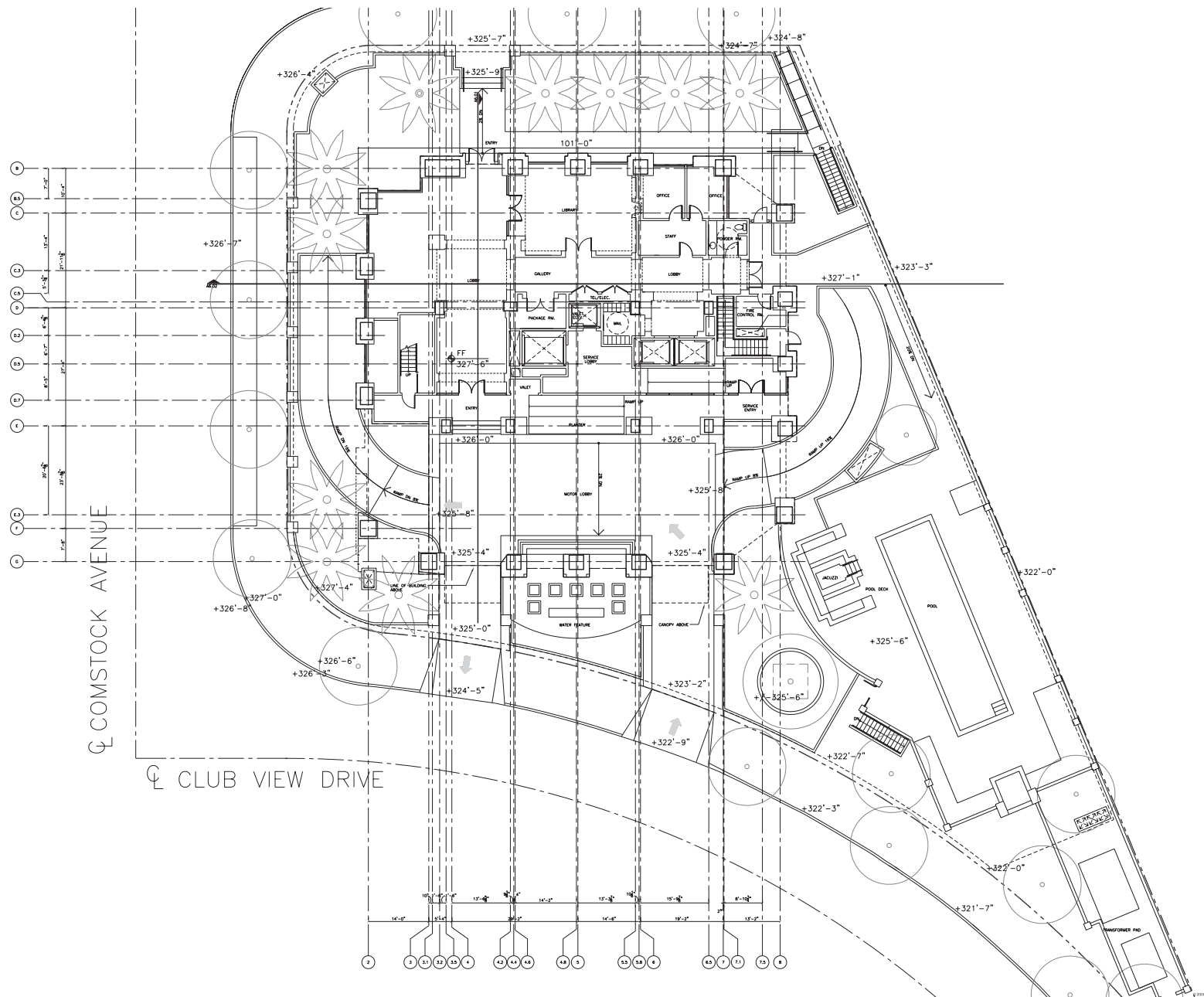
Figure III-1 Proposed Site Plan: 1st Floor
