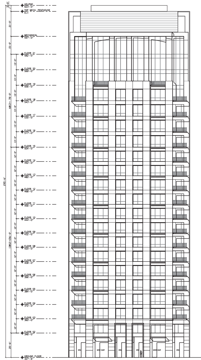
South Elevation
