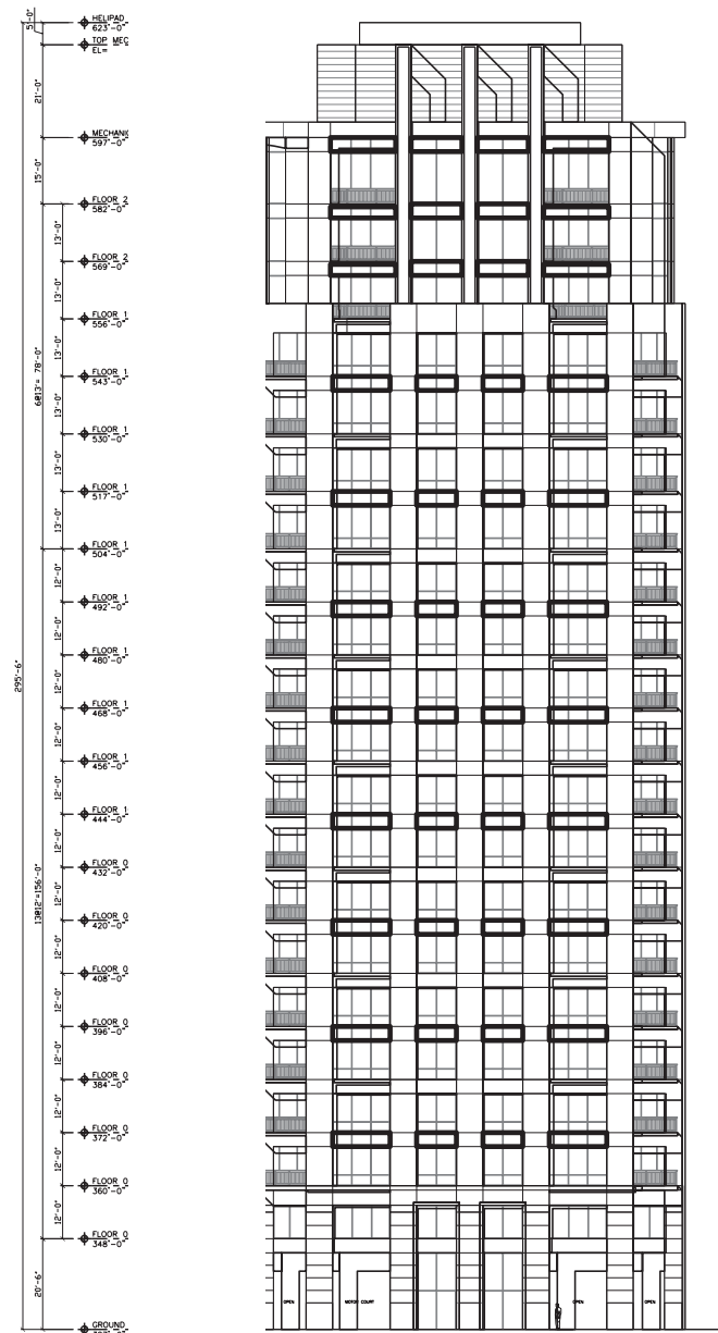
East Elevation
